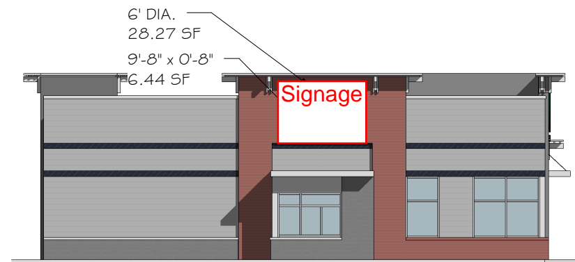
Side Elevation
